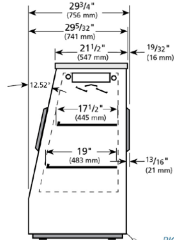
RIGHT VIEW
